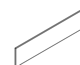
Wooden Modesty Panel + Hanging Bracket (2pcs) PX3 MP1200 - L 800 * W300 * T18mm PX3 MP1400 - L1000 * W300 * T18mm PX3 MP1500 - L1100 * W300 * T18mm PX3 MP1600 - L1200 * W300 * T18mm PX3 MP1800 - L1400 * W300 * T18mm
