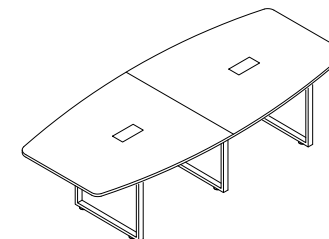
PX3 BS3000 Boat Shape Conference Table with Square Metal Legs L3000 * W1200 * H750mm
