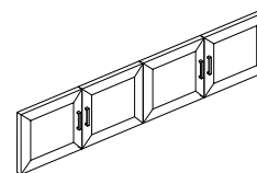
PX SH1800GD Glass Door with Aluminium Frame for PX3 SH1800 L445 * W392 * T20mm
