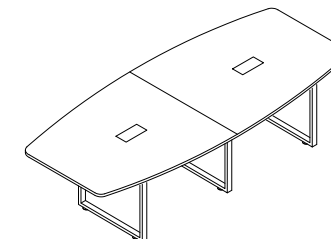
PX3 BS3600 Boat Shape Conference Table with Square Metal Legs L3600 * W1200 * H750mm
