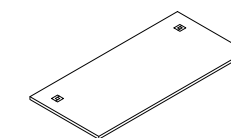
Standard Desk Top with 2 Grommets PX3 1200T - L1200 * W700 * T25mm PX3 1400T - L1400 * W700 * T25mm PX3 1500T - L1500 * W700 * T25mm PX3 1600T - L1600 * W700 * T25mm PX3 1800T - L1800 * W700 * T25mm
