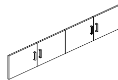
PX3 SH1800WD Wooden Door for PX3 SH1800 L445 * W392 * T18mm
