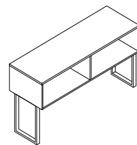
PX3 SH1800 Open Shared Hutch with Metal Support L1800 * W600 * H956mm
