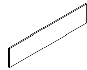
Wooden Modesty Panel + Hanging Bracket (2pcs) PX5 MP1200 - L 800 * W300 * T18mm PX5 MP1400 - L 1000 * W300 * T18mm PX5 MP1500 - L 1100 * W300 * T18mm PX5 MP1600 - L 1200 * W300 * T18mm PX5 MP1800 - L 1400 * W300 * T18mm
