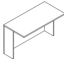
PX5 B1260W Bridge with Wooden Leg L1200 * W600 * H750mm
