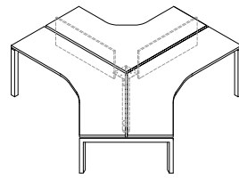
PX5 CC120JS 120° Joint Solution Universal Workstation with U-Hollow Metal Legs L2678 * W2320 * H750mm (Per Size : 2066 x 1105 x T25)
