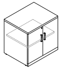
PX5 LC750 Low Cabinet with Wooden Door L700 * W400 * H750mm
