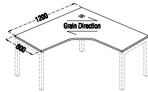
PX5 CC120T 120° Universal WorkTop L2079 * W1120 * T25mm
