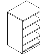
PX5 MHC1370 Medium Height Open Shelf Cabinet L800 * W400 * H1370mm
